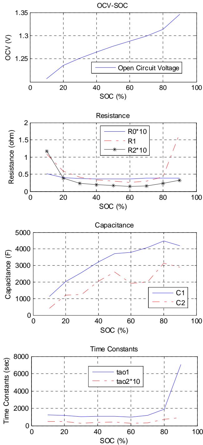
Figure 6 – Model Parameters as Functions of SOC .
