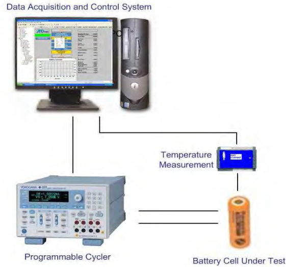
Figure 3 – Battery Test Setup.
